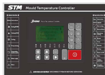
Control Panel
